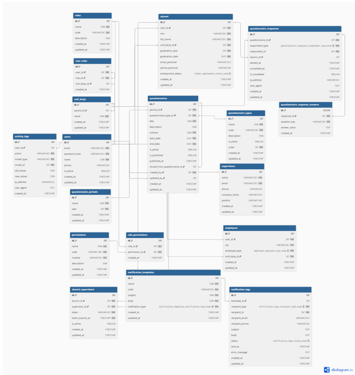
Gambar 3.11 Entity Relationship Diagram
